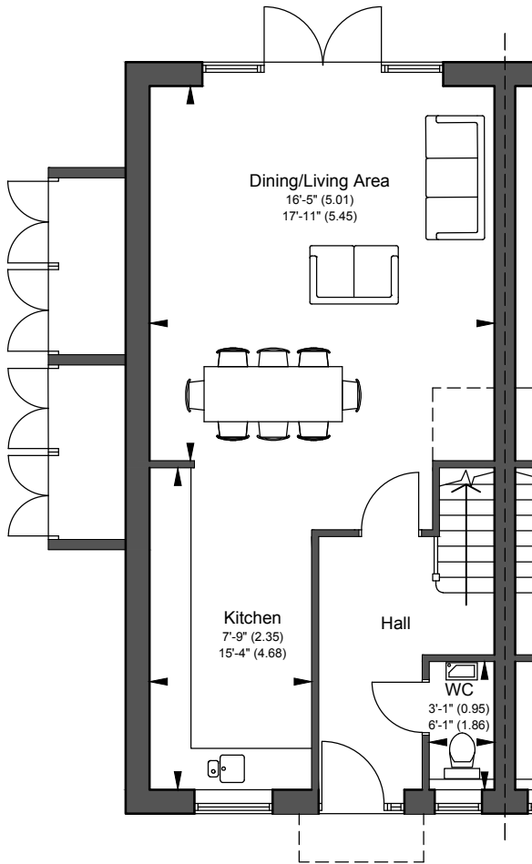
GROUND FLOOR PLAN PLOT 1
