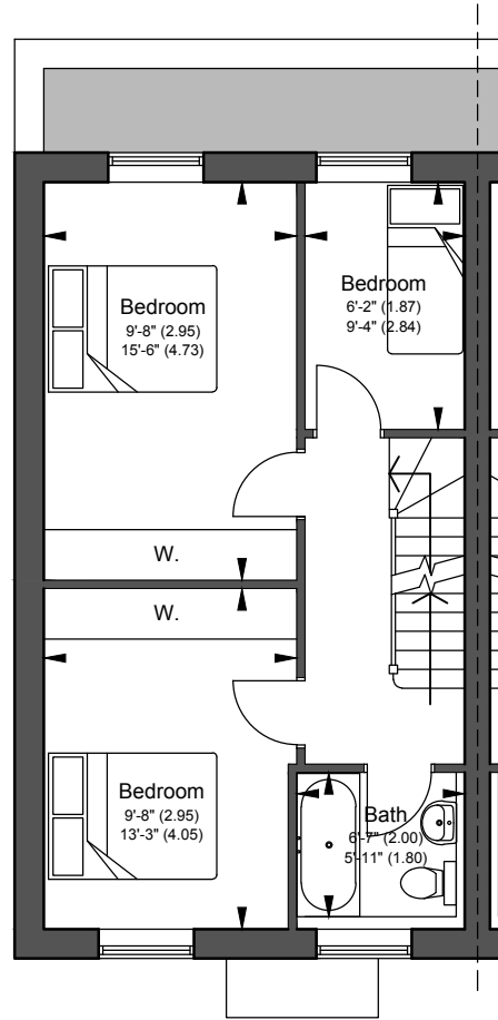
FIRST FLOOR PLAN PLOT 1
