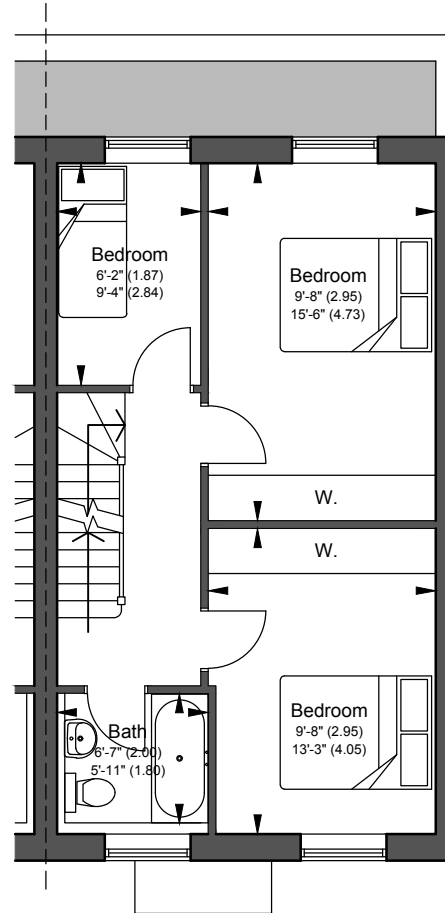
FIRST FLOOR PLAN PLOT 2
