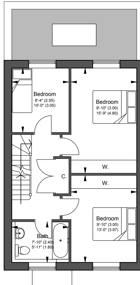
FIRST FLOOR PLAN PLOT 4
