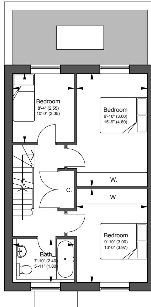
FIRST FLOOR PLAN PLOT 1
