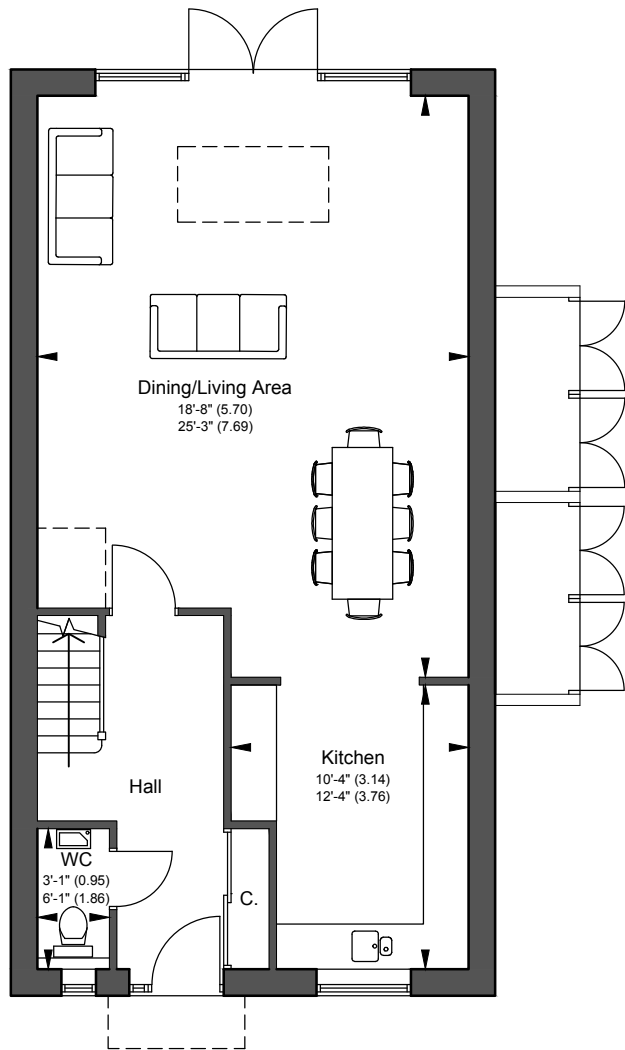
GROUND FLOOR PLAN PLOT 1
