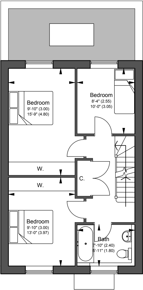
GF GIFA - 544.7ft 2 (50.6m 2 ) FIRST FLOOR PLAN PLOT 2
