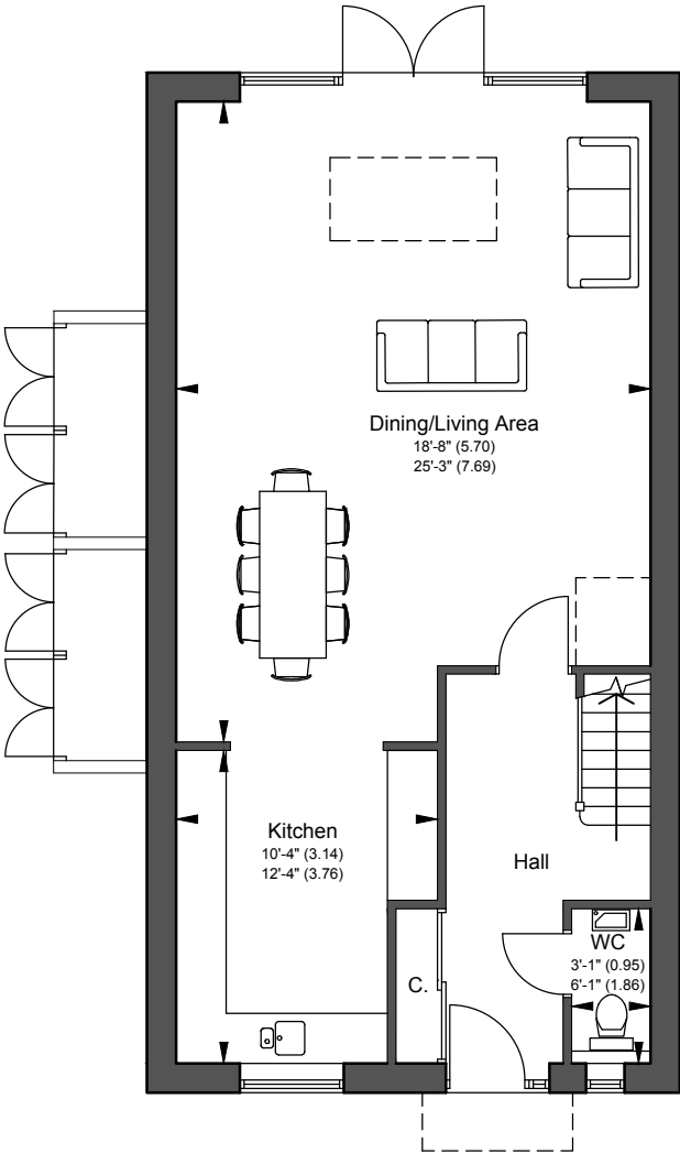
GF GIFA - 718.0ft 2 (66.7m 2 ) GROUND FLOOR PLAN PLOT 2
