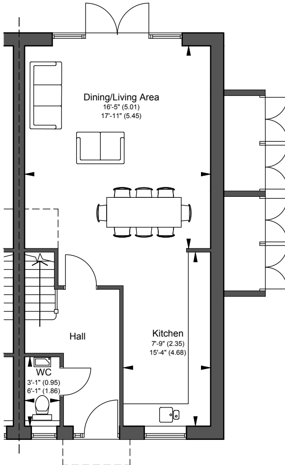
GROUND FLOOR PLAN PLOT 3
